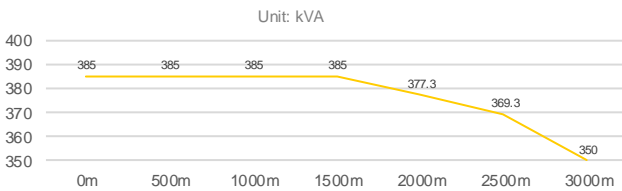
Altitude (meters) Derate Curves
