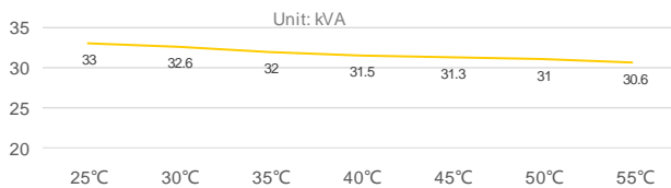
Temperature (Celsius) Derate Curves
