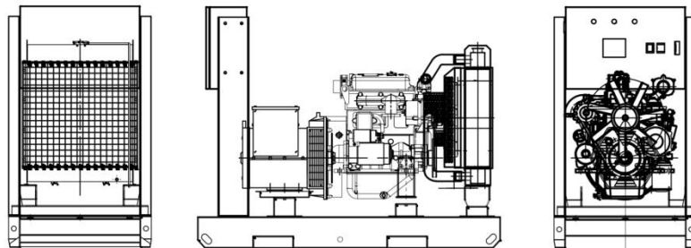
LSP14E3 (开架式)
