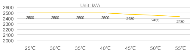
Temperature (Celsius) Derate Curves
