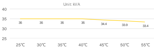
Temperature (Celsius) Derate Curves
