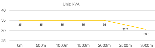
Altitude (meters) Derate Curves
