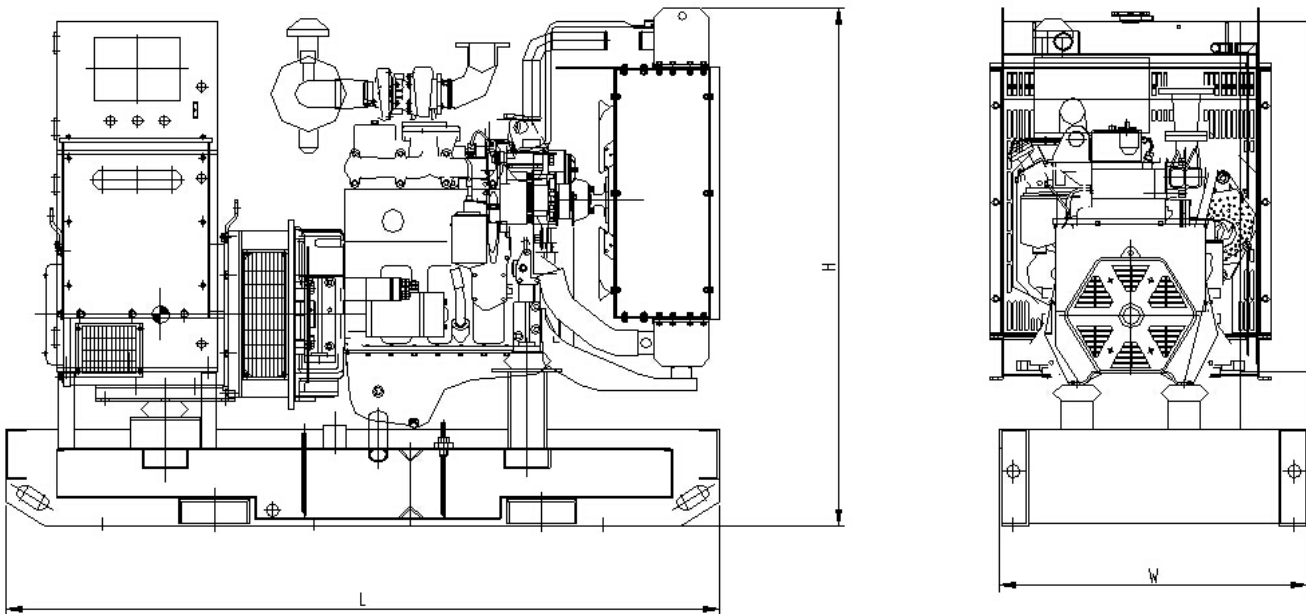
LSC24E3 (Open type)
