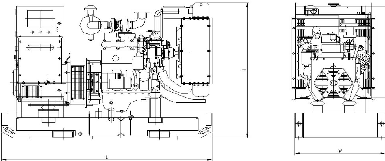
LSP500E3 (Open type)
